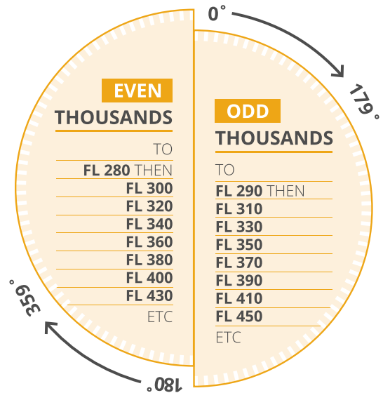
Figure 14: Specified IFR cruising level – at or north of 80 degrees south
