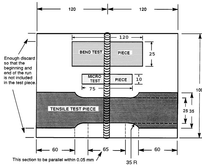
Diagram 1 – Joint No 1 – Sheet to Sheet Butt Weld
