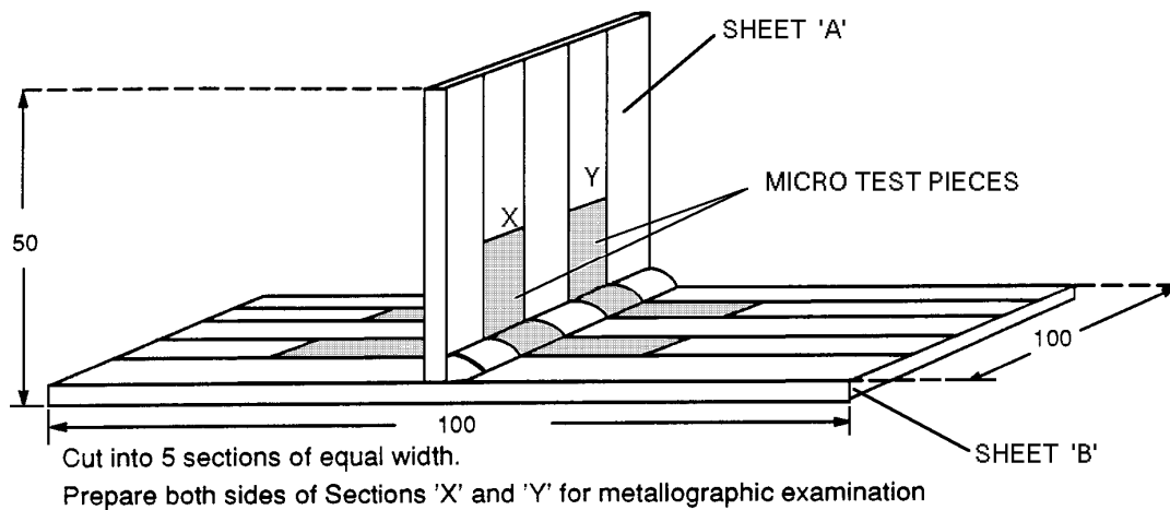
Diagram 3 – Joint No 3 – Sheet to Sheet Fillet Weld
