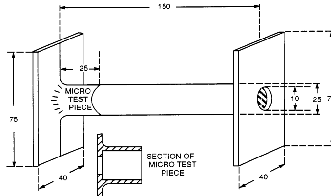
Diagram 2 – Joint No 2 Sheet to Tube Fillet Weld
