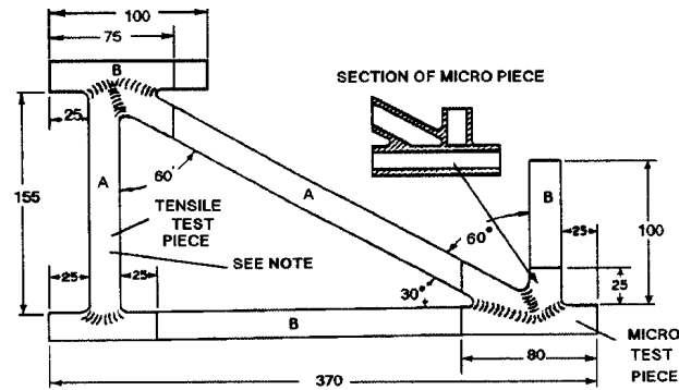
Diagram 4 – Joint No 4 – Tube To Tube Weld
